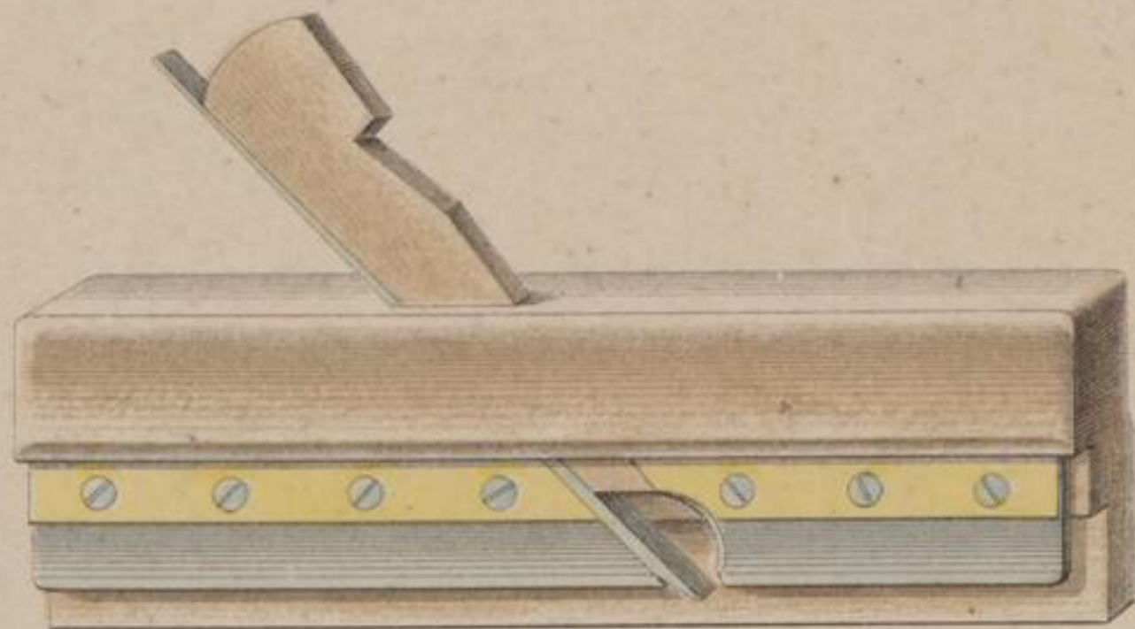
Nuthobel
