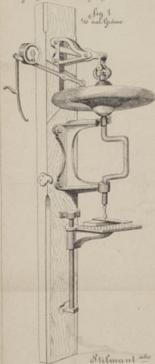
Patent Bohrmaschine Lyon & Co. in New York
