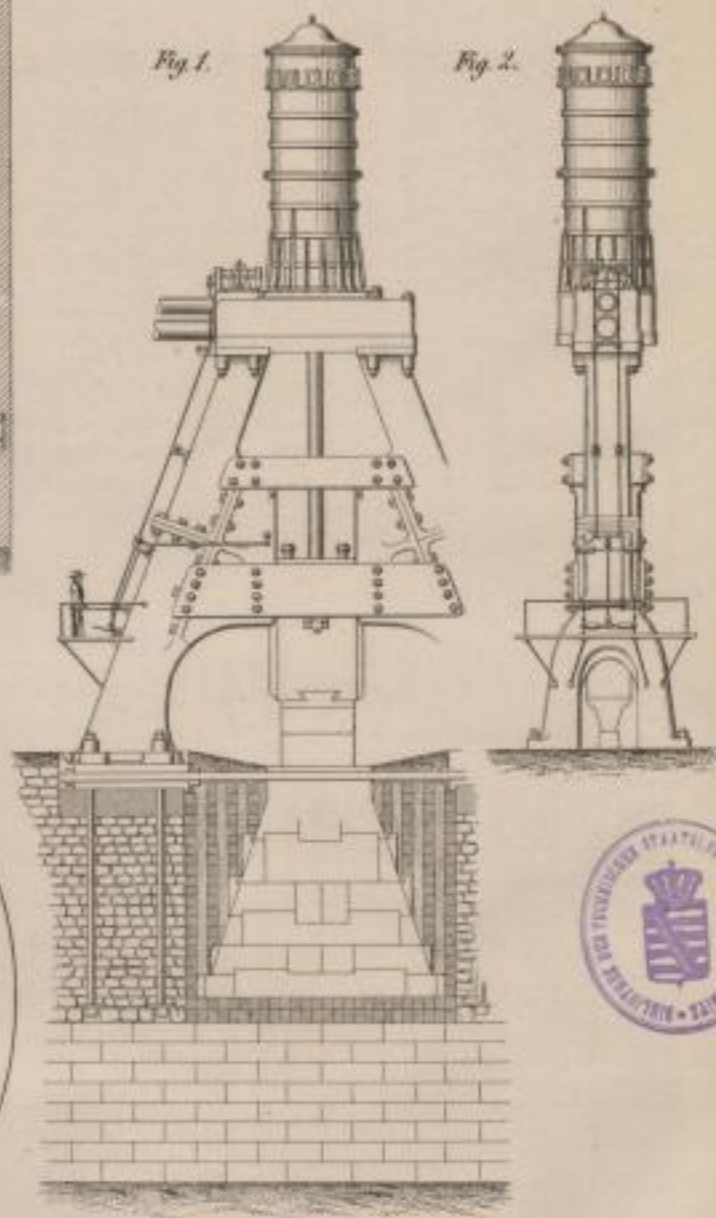
80-Tonnen-Dampfhammer in Creuset (Fig. 1, 2).
