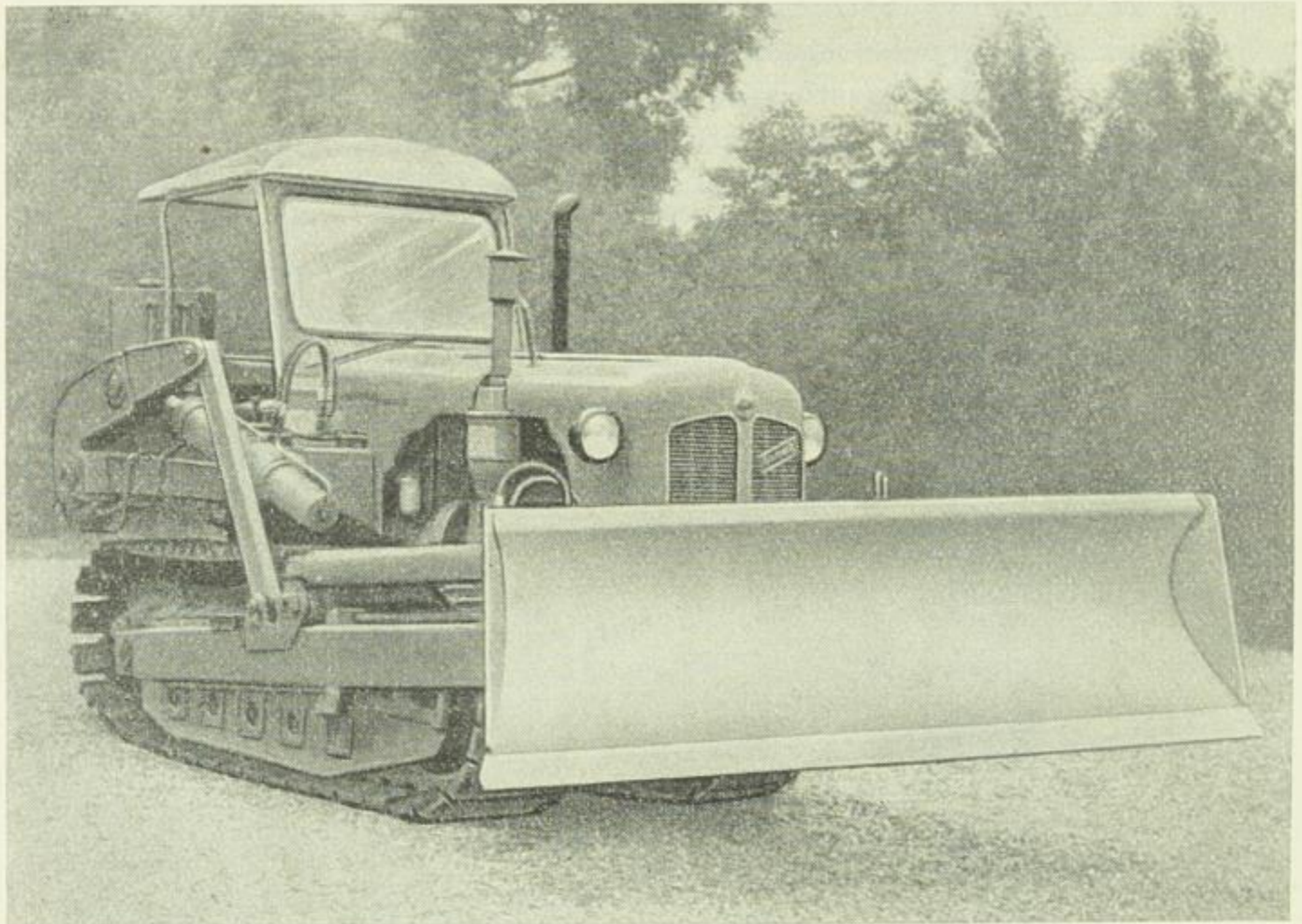
Fig. 8. Crawler tractor with attached pusher-blade ready for use in the construction industry (Type: KT 50 / output up to 70 m 3 /h at a travelling distance of 10 m / speed 3.0 to 6.6 km/h.)
