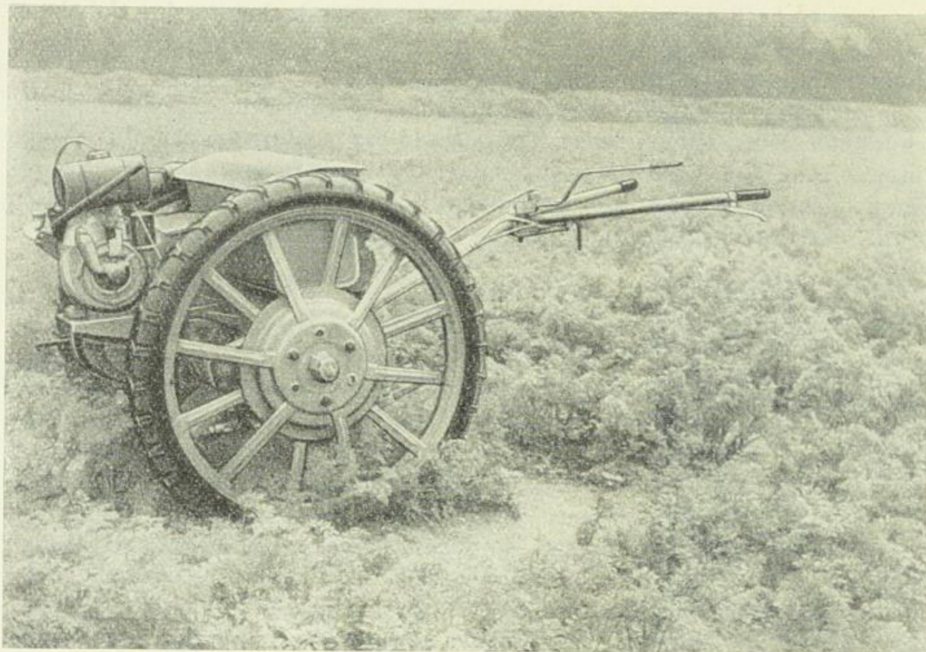
Fig. 30. Two-wheel tractor (Two-stroke petrol engine / 1 cylinder 143 m 3 swept volume / 3.5 h.p. - Manufacturer: Saxonia Bernburg)
