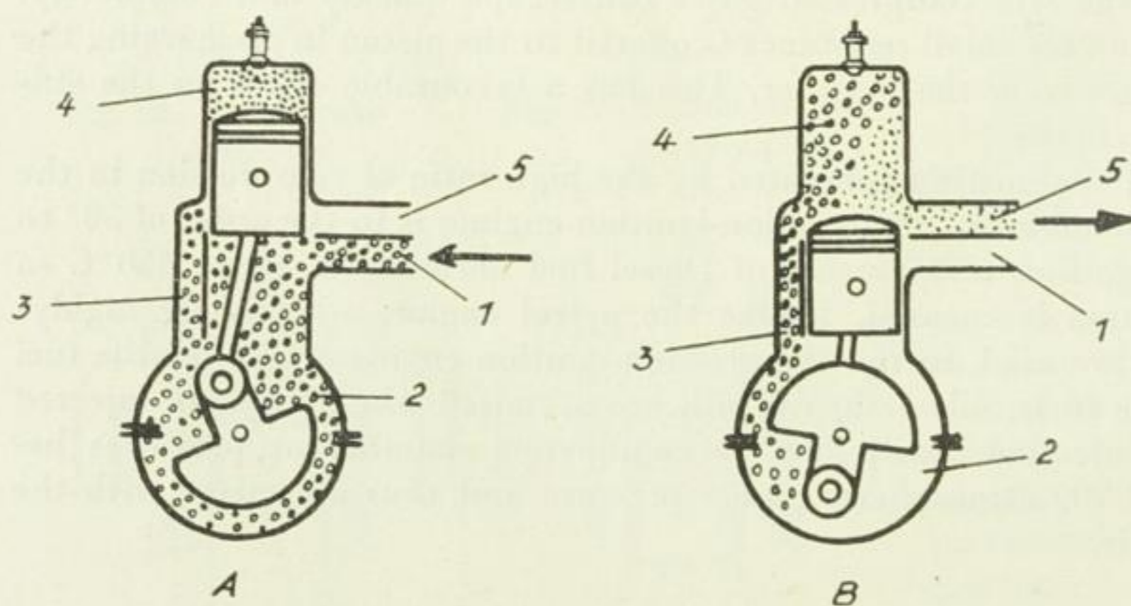
Fig. 31. Cycle of the two-stroke petrol engine
