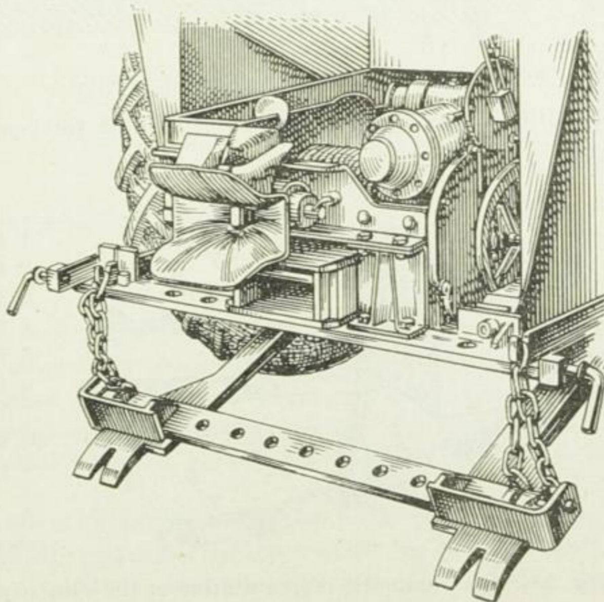
Fig. 302. Attachment rail with sprags
