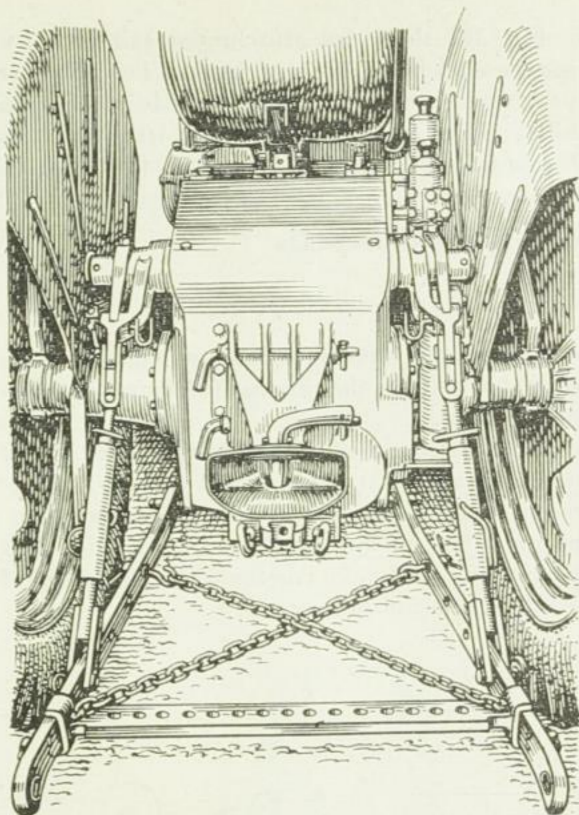
Fig. 301. Attachment rail with hydraulic lifting device (power lifter); bracing chains are diagonally arranged
