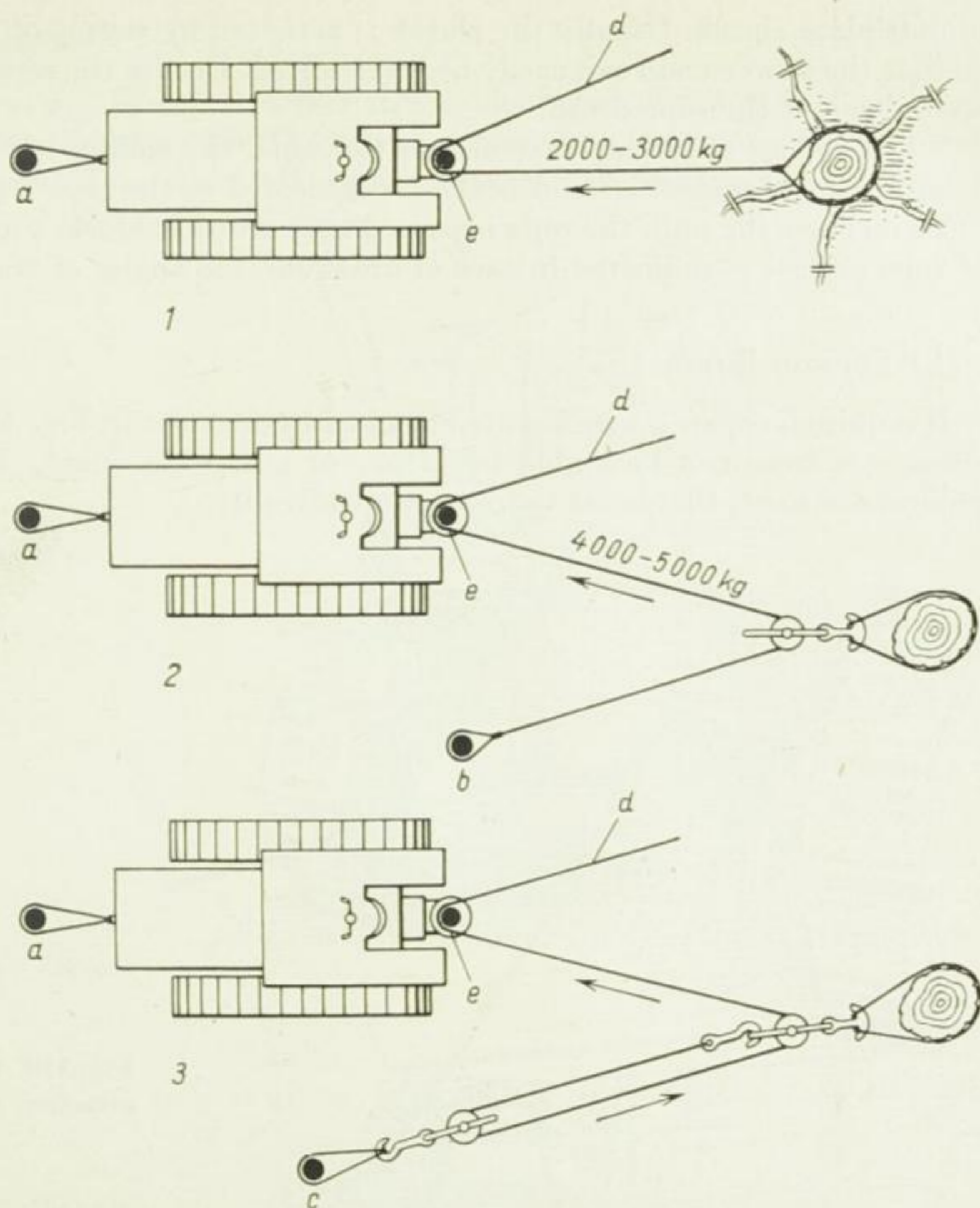
Fig. 309. Work performed by means of a capstan winch
