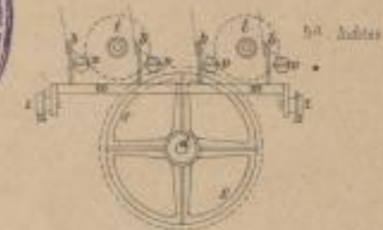
Stein's Kartchen-Bewickel-Maschine.
