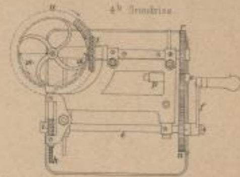
Stein's Kartchen-Bewickel-Maschine.
