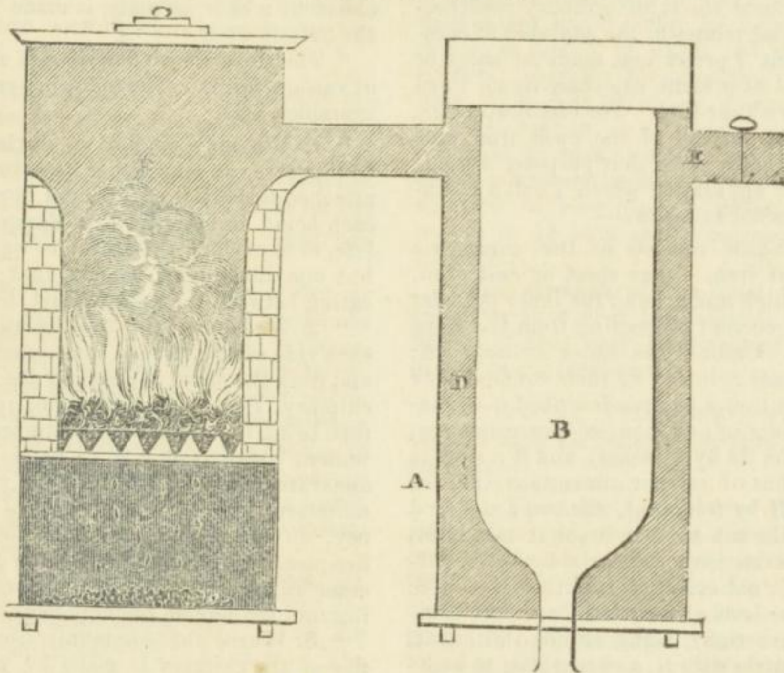
OLMSTED'S STOVE.
