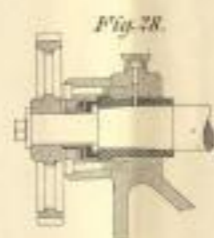
Sellers' Supportdrehbank.
