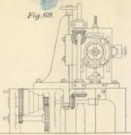
H. Hind & Son. Horizontalbohrmaschine.
