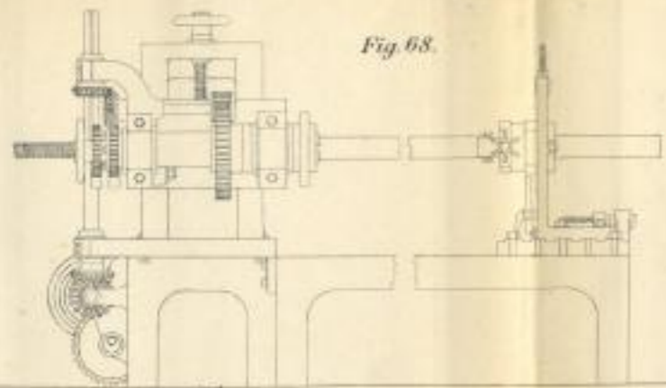
H. Hind & Son. Horizontalbohrmaschine.
