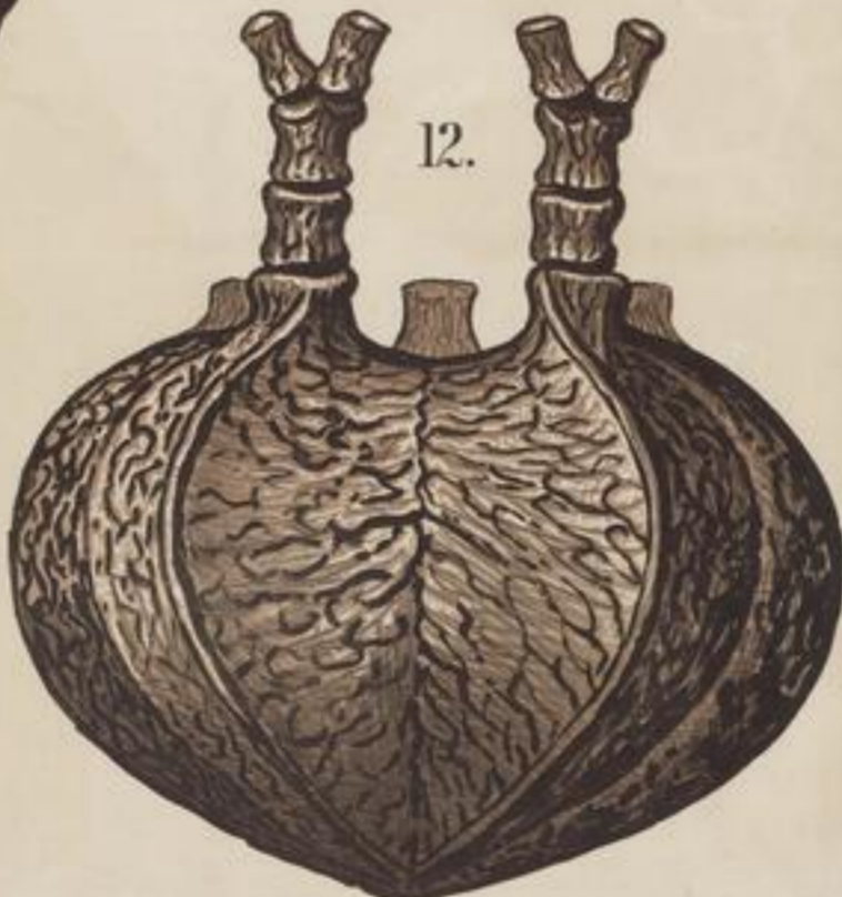
1. Rhodocrinus quinquelobus 2. Marsupites ornatus. 3. 4. Encrinus liliiformis. 5. Millericrinus magnificus 6. Millericrinus tuberculatus 10. Solanocrinus co 7. Apiocrinus Parkinsoni. 9. Pentacrinus status. 11. 12. Saccocoma pectinata. 8. Eugenicrinus caryophyllatus.
