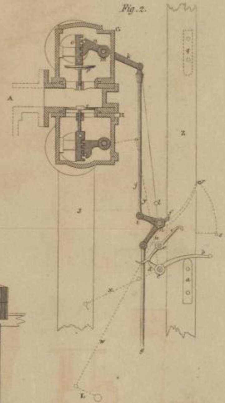
Manner of Opening and Shutting the Nozzle Valves.
