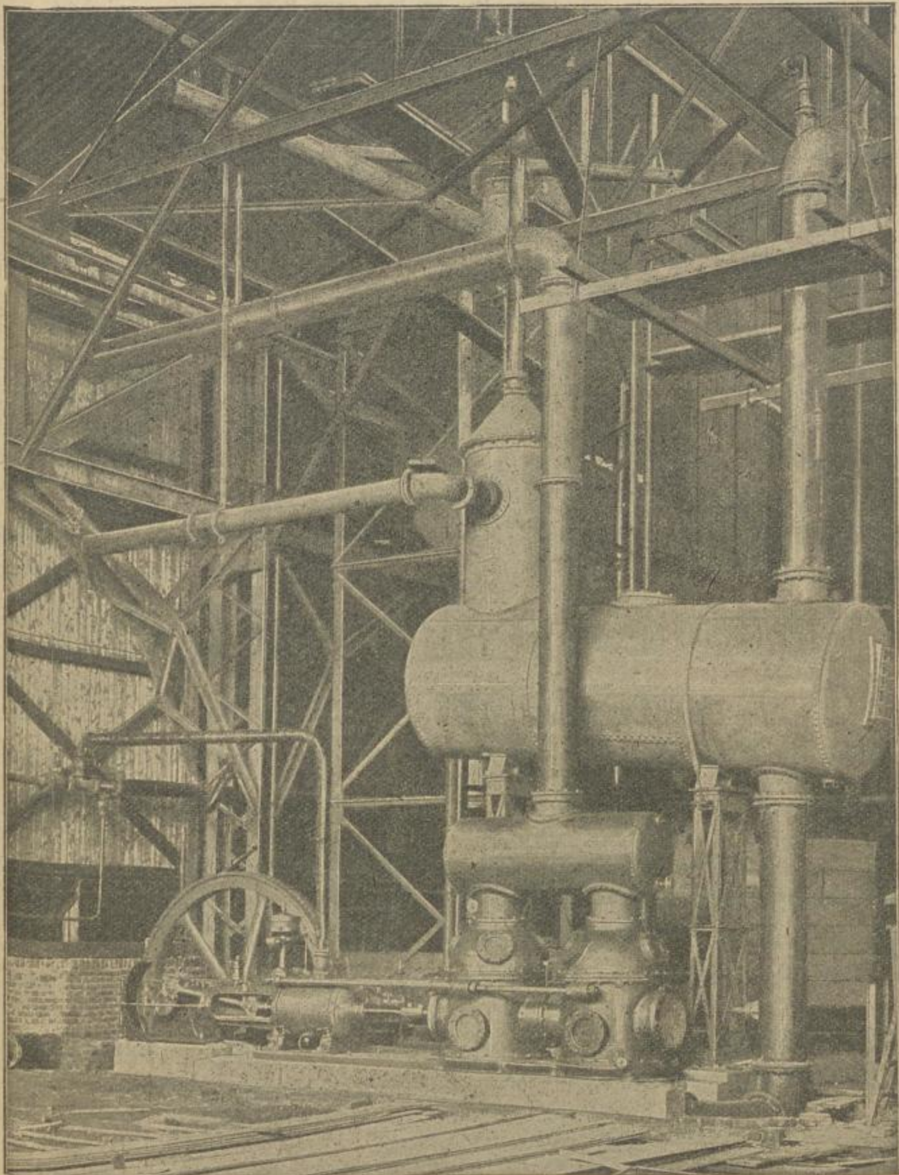
Neues System. Central-Einspritz-Condensation System Schwarz.
