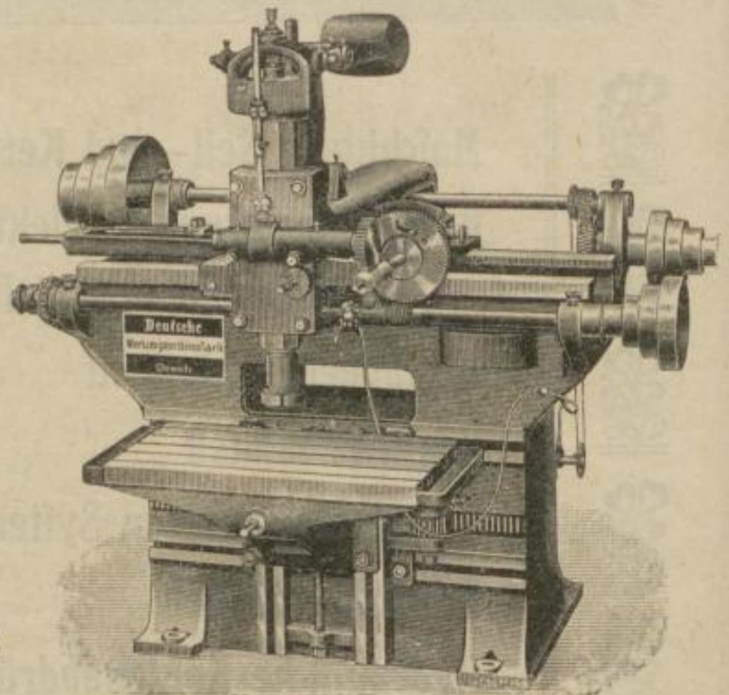
Langloch-Bohrmaschine.
