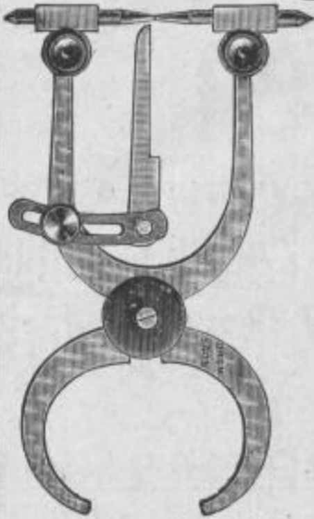
Parallel-Rundlaufzirkel, System Beck. Mk. 2,60.
