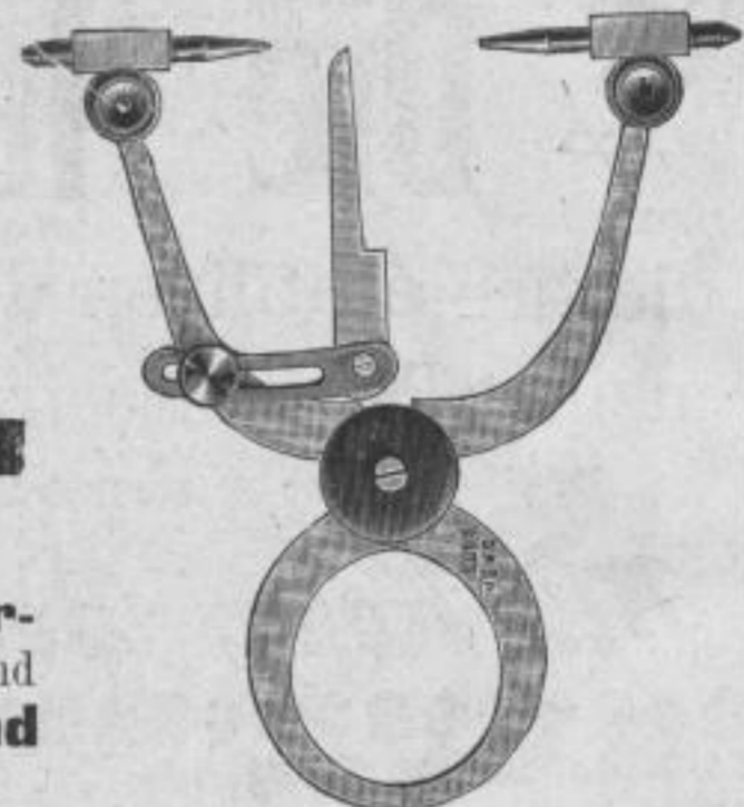
Parallel-Rundlaufzirkel, System Beck. Mk. 2,60.
