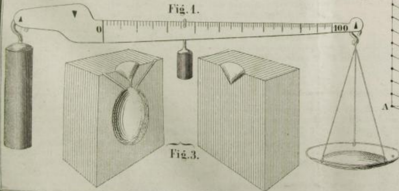
Place's Zinnwage.
