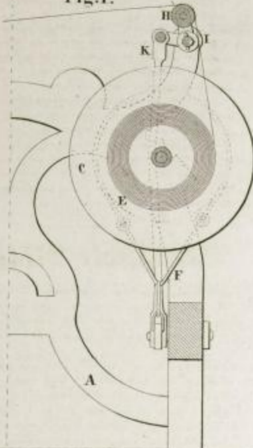
Mouline's Regulator.
