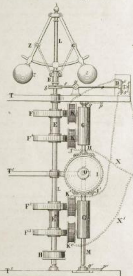
Mouline's Regulator.
