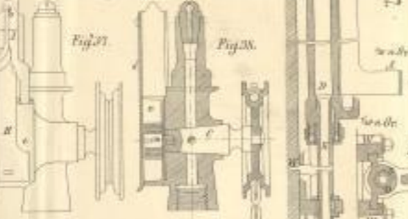
Folding and Platt's Krahn (177-178)
