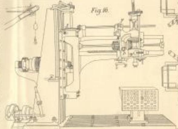
Asquith's Radialbohrmaschine (177)
