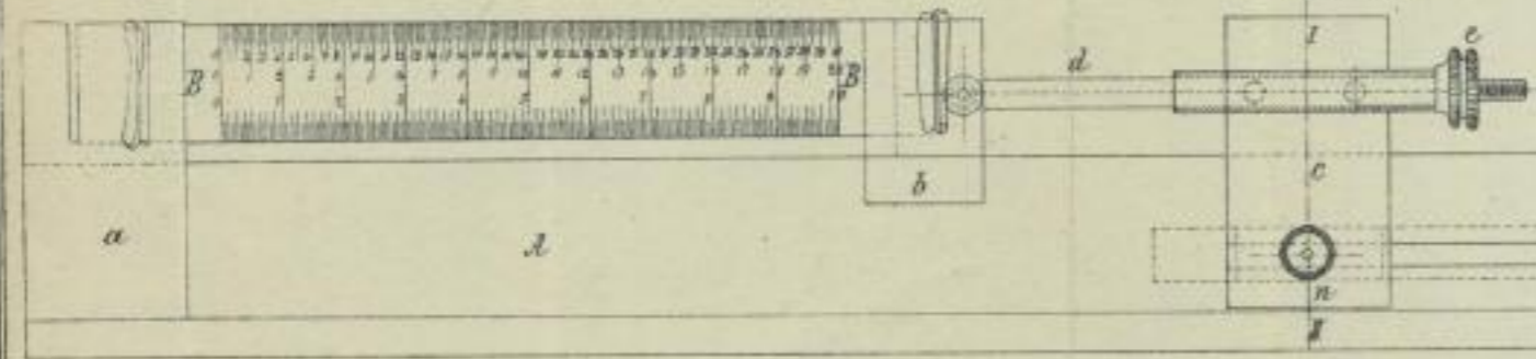
Fig. 6. André's Theilapparat. (6-8)
