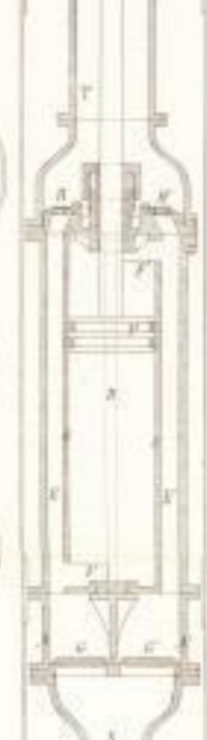
Lynde's Aestapparat
