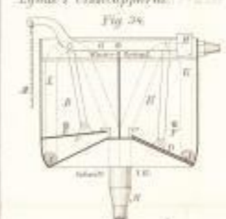
Lynde's Aestapparat
