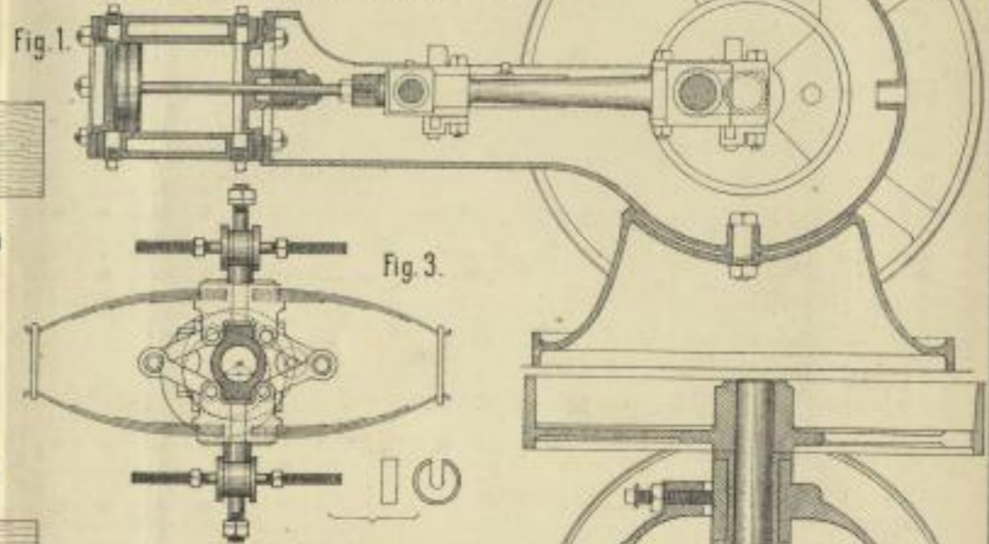
Huntoon's Dampfmaschine. (1-3)
