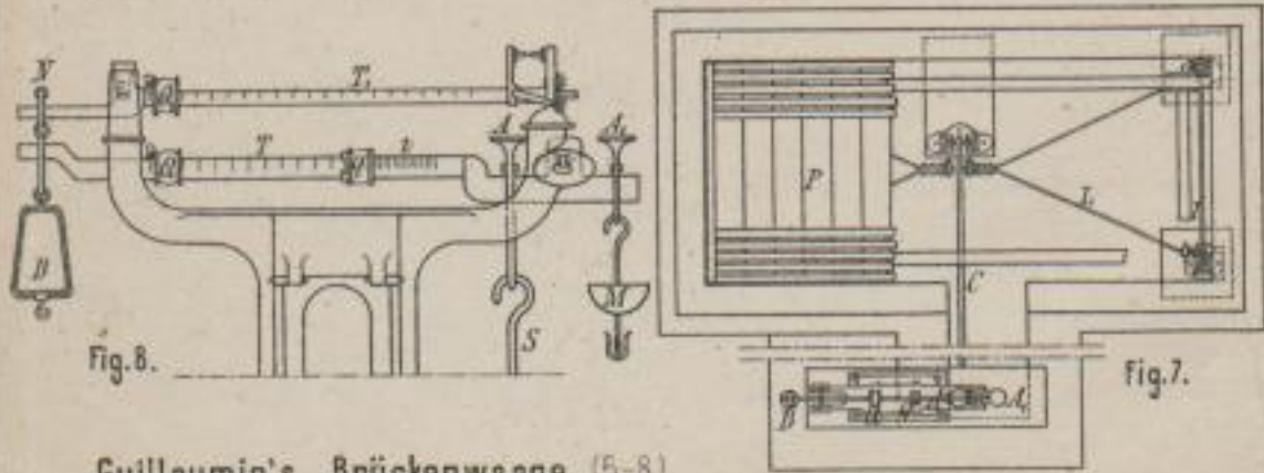
Guillaumin's Brückenwaage. (5-8)
