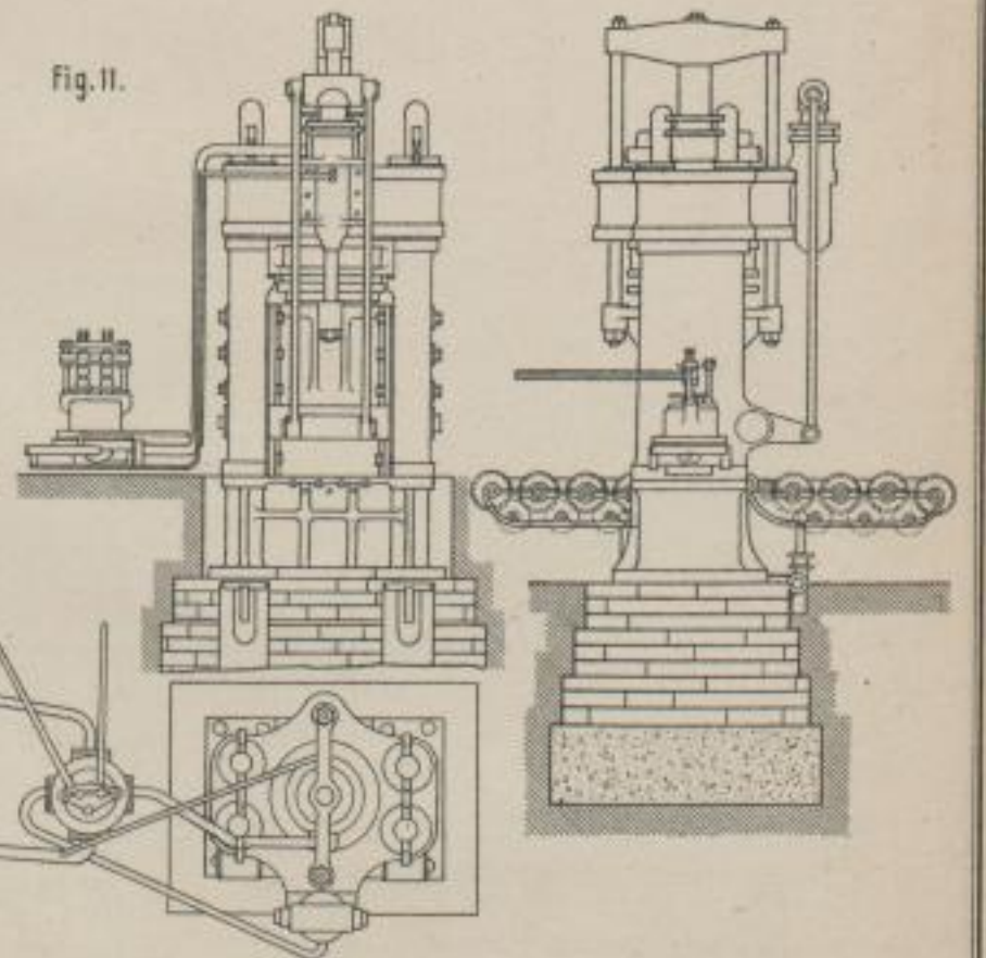
J. Copeland's Blockschere. (11 u. 12)
