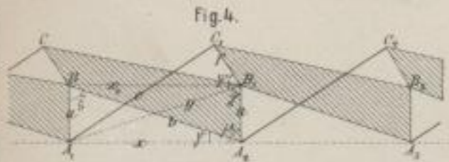
Toulmin's Ellipsograph. (13)
