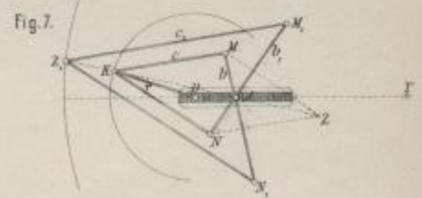
Peaucellier's Zirkelparallelogramm. (5-7)
