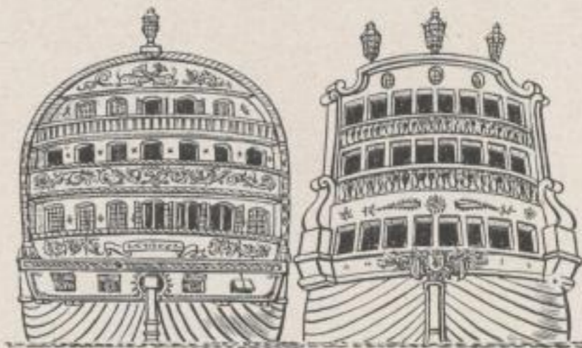
Illustrations for "Schiffsibel"
