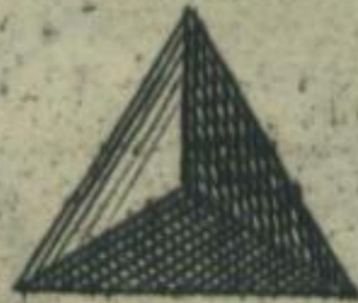
Tetraedrum
