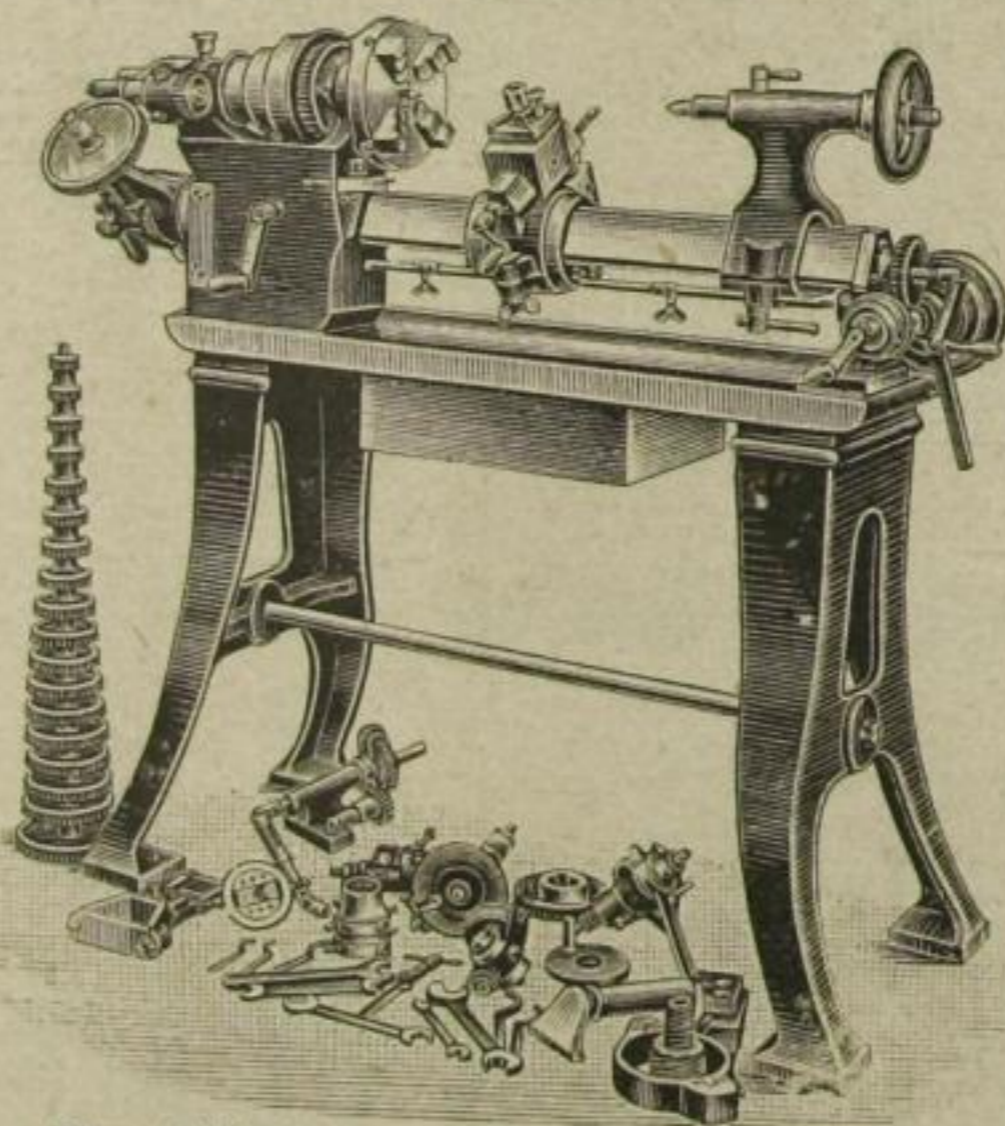
W. v. Pittler's Patent-Drehbank, Modell C. III.
