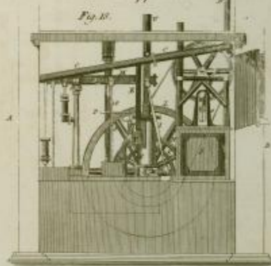
Davy's Dampfmaschine.
