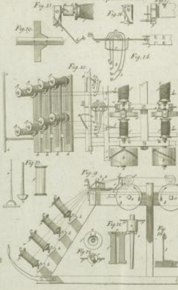
Skotten's Seiden Spinnmaschine
