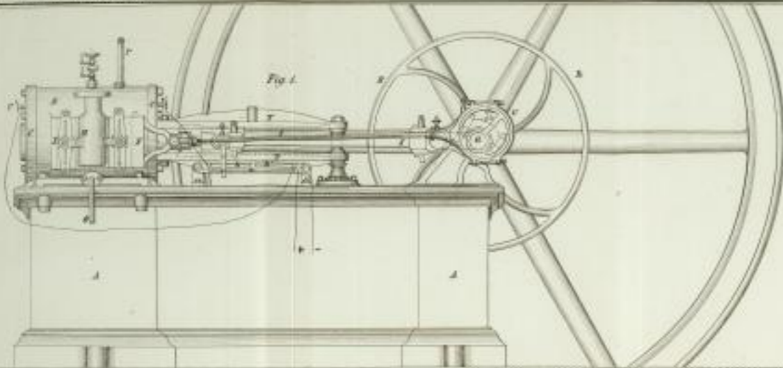
Lenoir's Gasmachine.
