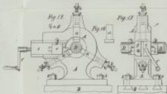
Klein's Lunette-Support.
